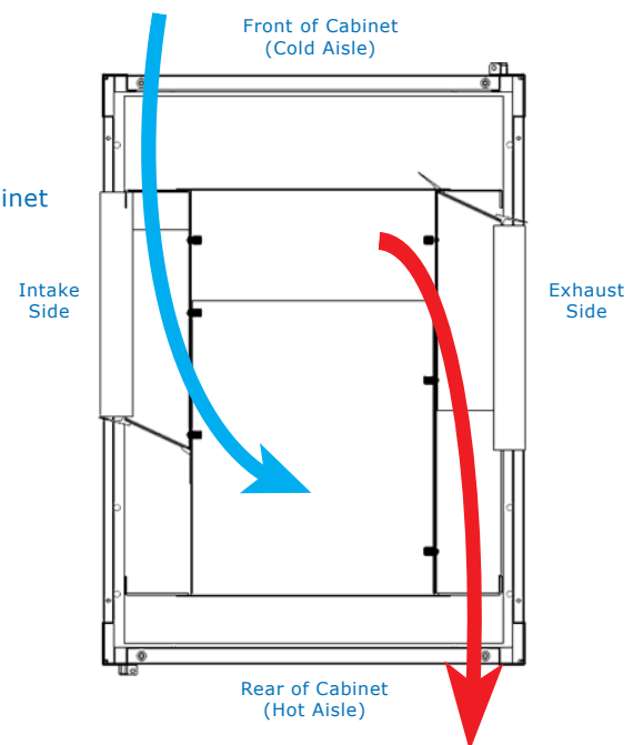
TOP VIEW OF SIDE VENT READY CABINET
