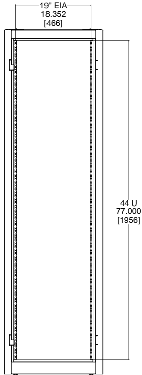
FRONT VIEW DOORS REMOVED
