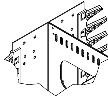
DETAIL A HARDWARE USAGE (BULK PKG AND STRAP TO MANAGER)
