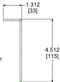
DETAIL A SCALE 3 : 1
