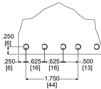
DETAIL B SCALE 6 : 1
